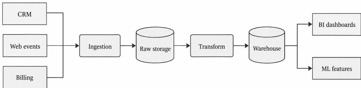
Figure 2. Data platform overview
